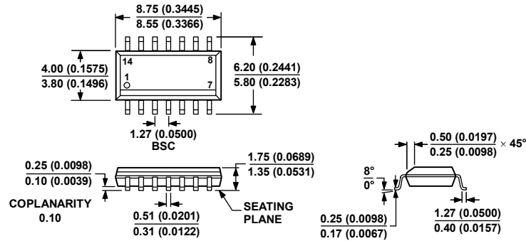
Figure 38. 14-Lead Standard Small Outline Package [SOIC_N] Narrow Body (R-14) Dimensions shown in millimeters and (inches)
