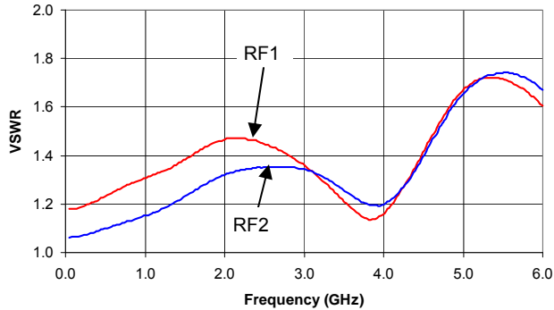
VSWR - 8 dB Bit vs. Frequency
