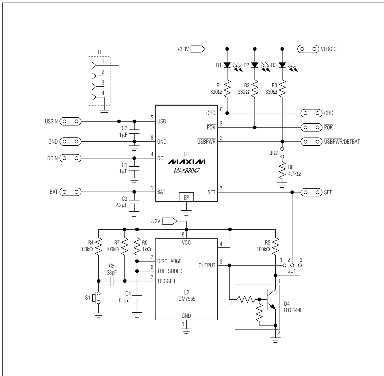
Figure 1. MAX8804Z EV Kit Schematic
