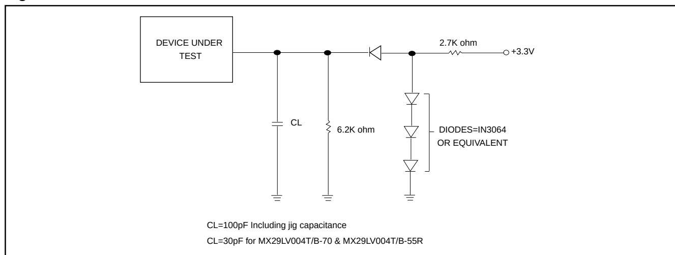
Figure 1. SWITCHING TEST CIRCUITS
