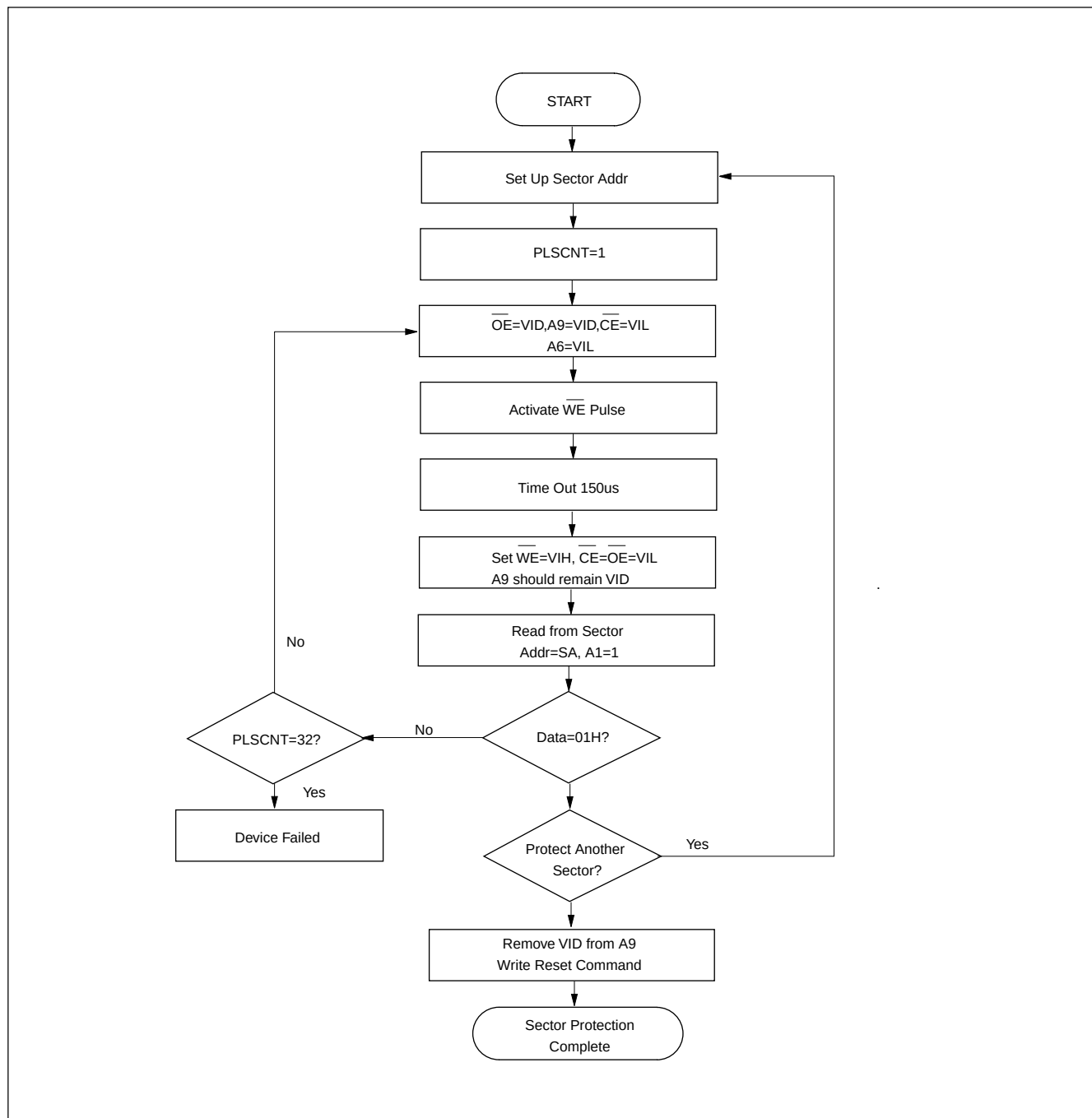
Figure 16. SECTOR PROTECTION ALGORITHM (A9, \overline{OE} Control)
