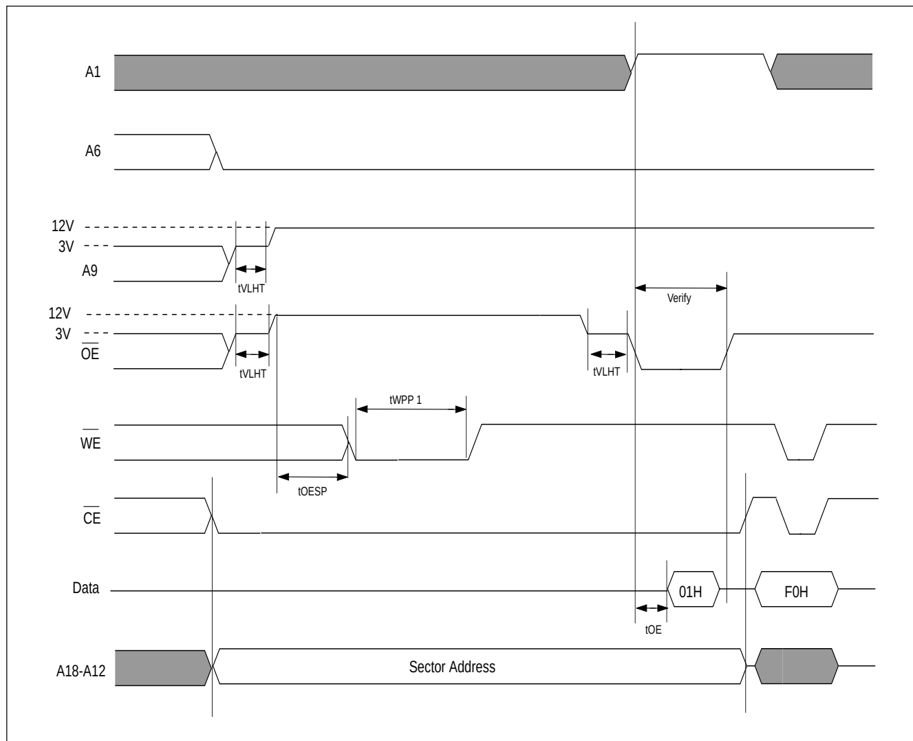
Figure 15. SECTOR PROTECT TIMING WAVEFORM(A9, \overline{\text{OE}} Control)
