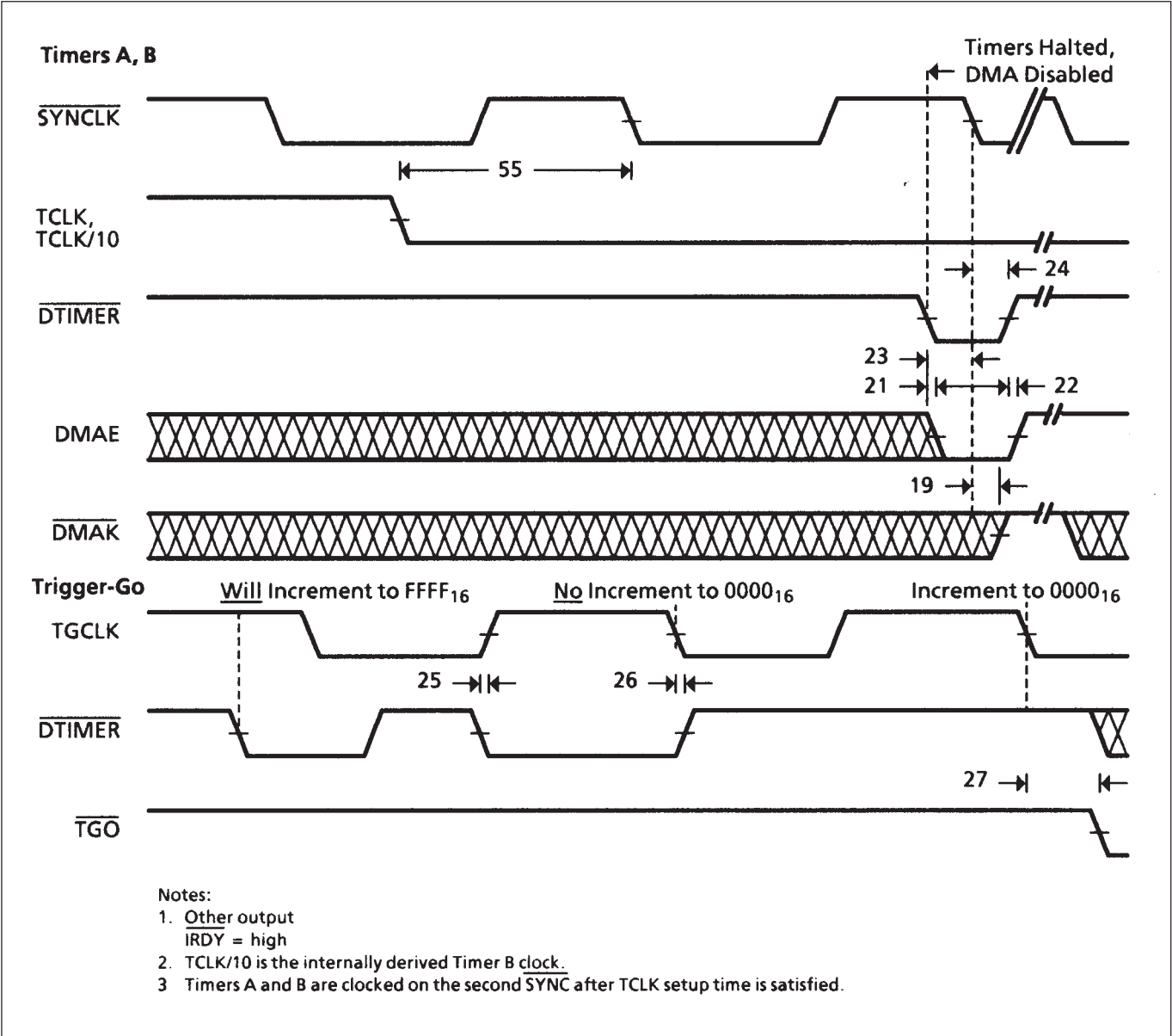
Figure 15: Timer Operations
