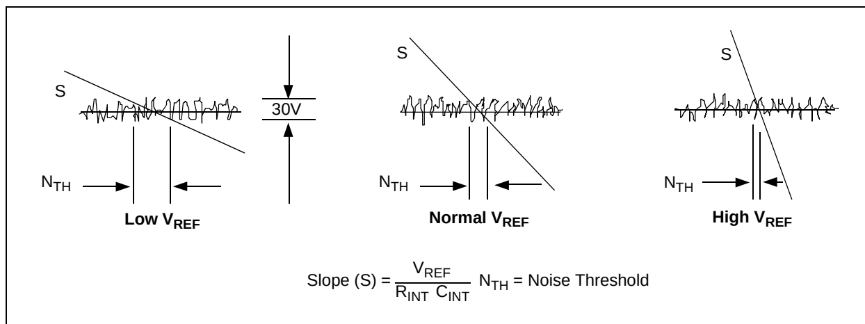
FIGURE 8-1: Noise Threshold.
