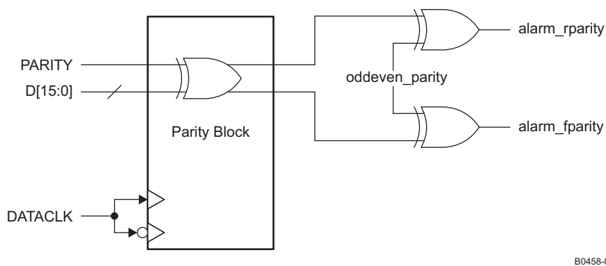
Figure 79. DAC3484 Word-by-Word Parity Check
