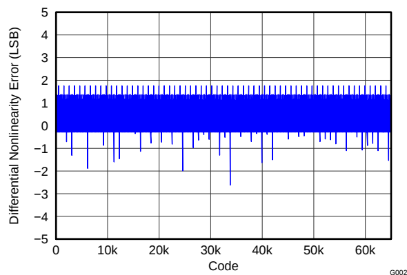
Figure 2. DIFFERENTIAL NONLINEARITY
