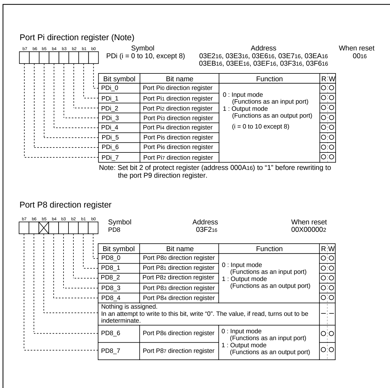
Figure 1.20.6. Direction register
