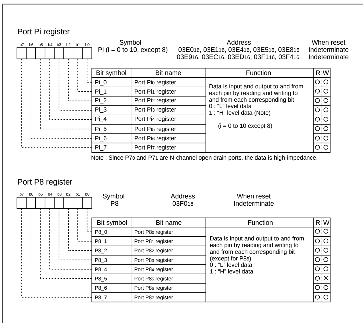
Figure 1.20.7. Port register
