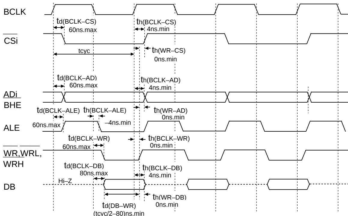
Figure 1.23.9. V_{CC}=3V timing diagram (3)
