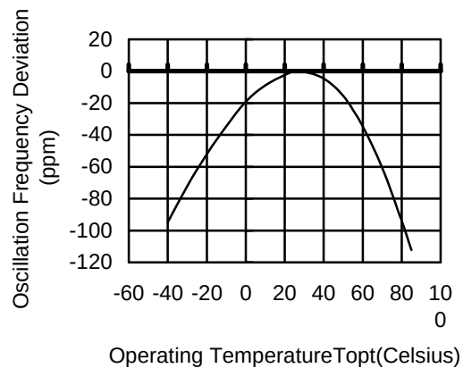
Oscillation Frequency Deviation vs. Operating Temperature ( V_{DD}=3V , T_{opt}=25^{\circ}C as standard)
