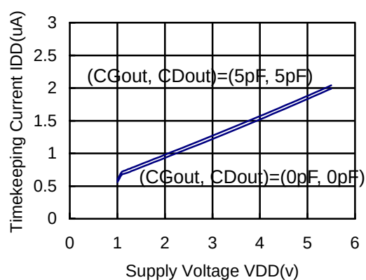
Timekeeping Current vs. Supply Voltage (with 32kHz clock output) (Output=Open, Topt=25°C)
