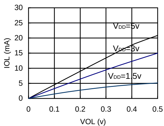
V_{OL} vs. I_{OL} ( \overline{INTR} pin) ( T_{opt}=25^{\circ}C )
