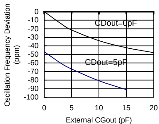
Oscillation Frequency Deviation vs. External CGout ( V_{DD}=3V , T_{opt}=25^{\circ}C , CG_{out}=CD_{out}=0pF as standard)
