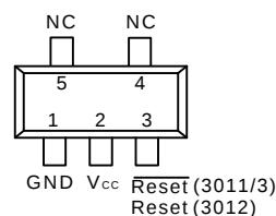
SOT-23-5 (Top View)
