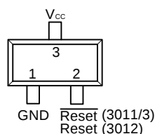
SOT-23-3 (Top View)
