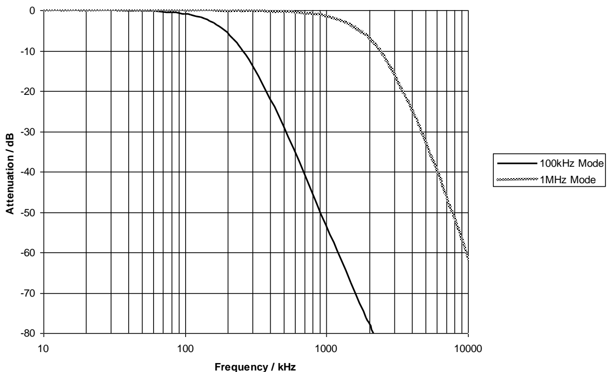
Figure 27 Typical Receiver I/Q Frequency Response
