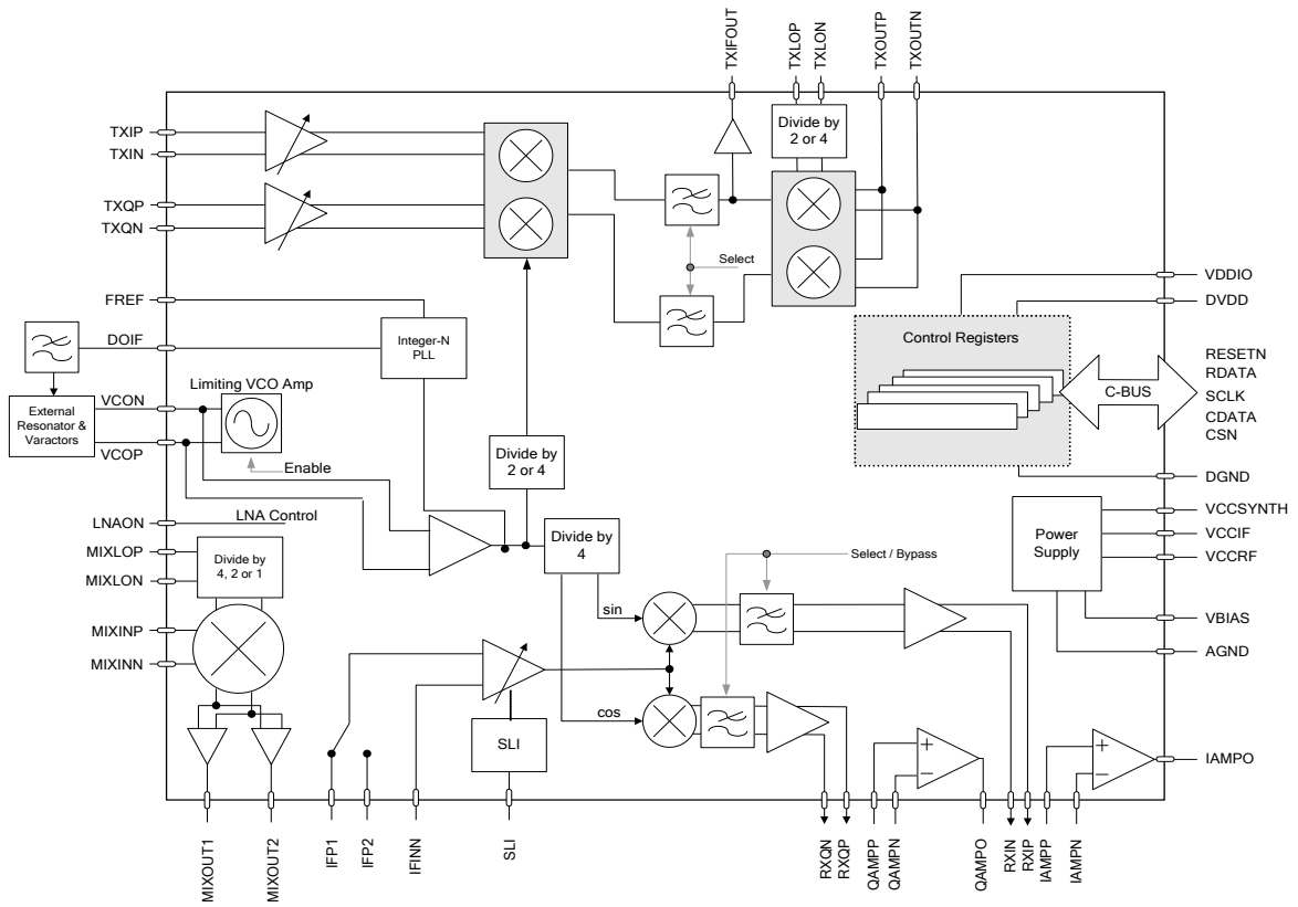
Figure 3 CMX991 Block Diagram
