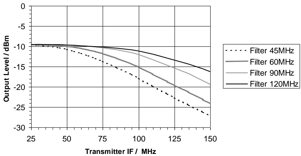
Figure 30 Transmitter IF Output Showing Filter Responses with IFH bit = '1'
