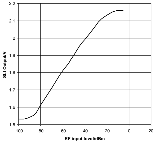
Figure 25 Typical SLI Performance in an Application Circuit (EV9920B) (Input 460MHz, 25kHz IF crystal filter: 45G15B1)
