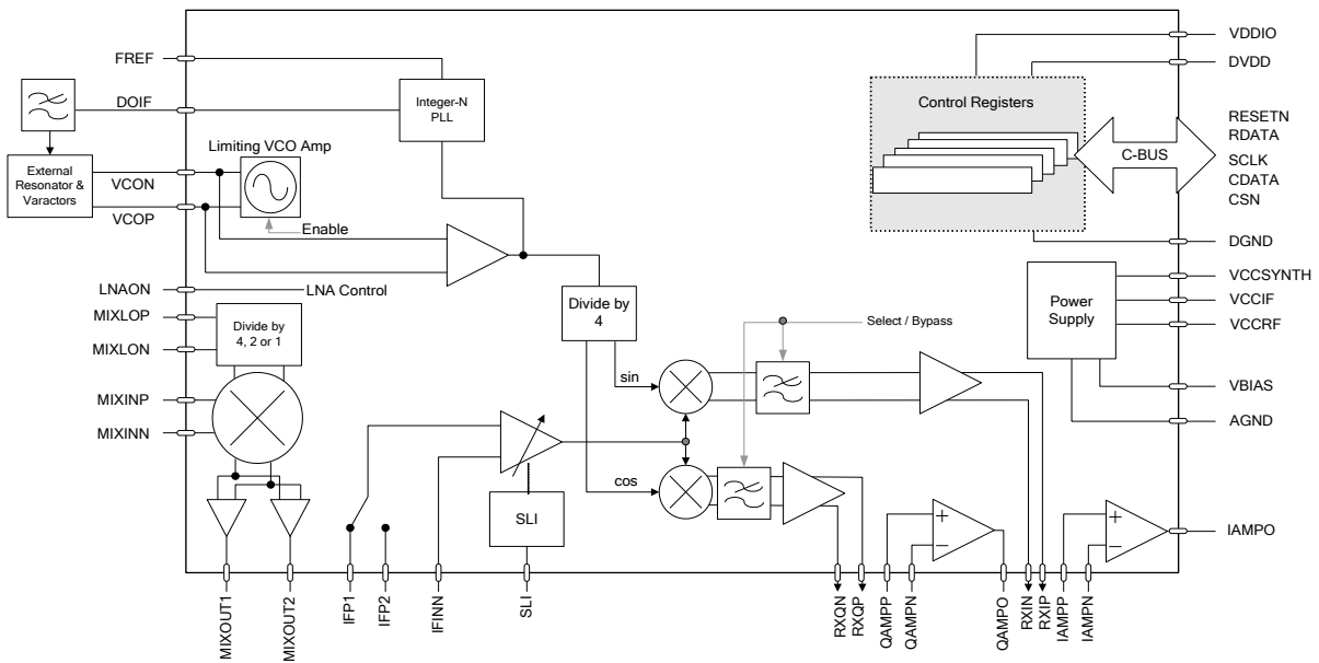
Figure 3 CMX991 Block Diagram
