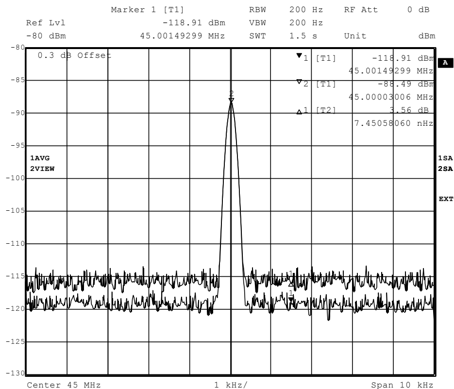
Figure 26 IF Output Response with and without Blocking Signal Present
