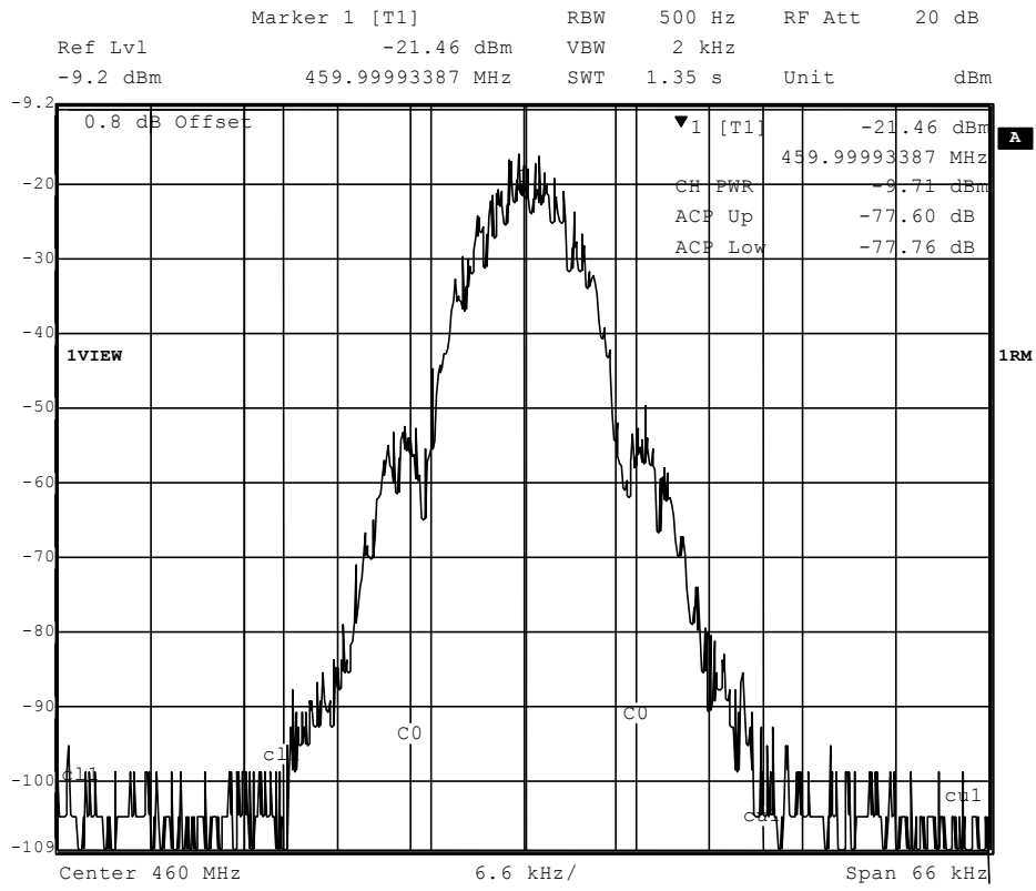
Figure 28 Tx Output with 9.6kbps GMSK from an EV9100 (TxIF = 90MHz, ACP ~ 77dBc)
