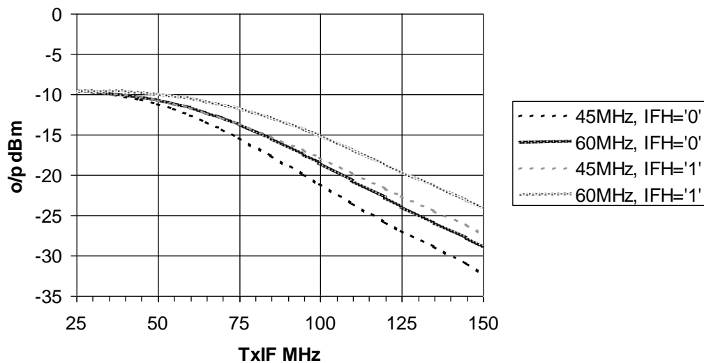
Figure 31 Effect of IFH on 45MHz and 60MHz Transmitter IF Filters
