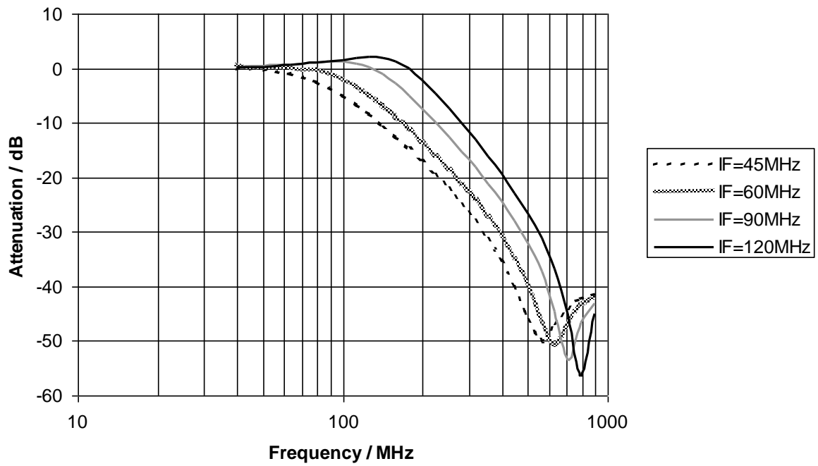
Figure 29 Transmitter Path IF Filters
