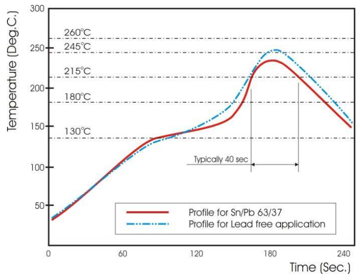
Fig 3. Infrared soldering profile for chip resistor
