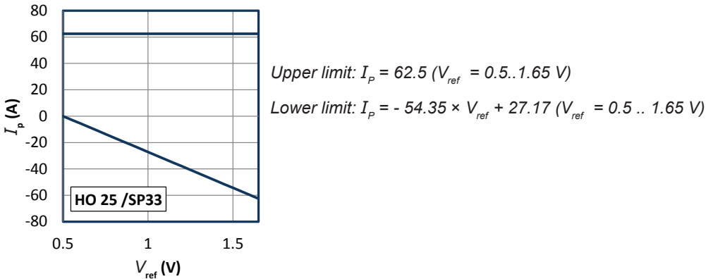
Figure 17 I_p vs V_{ref} for HO/SP33 series
