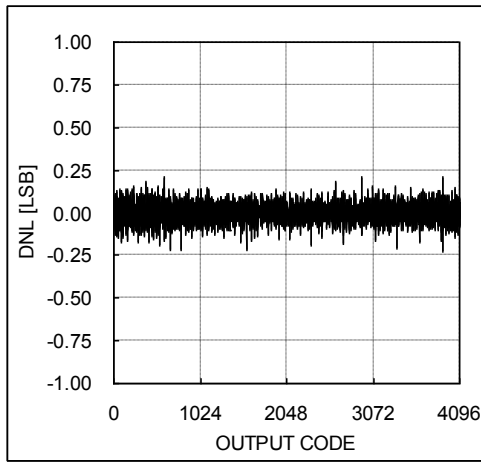
Figure 8. DNL vs OUTPUT CODE ( V_A=3\text{V} , f_{SCLK}=20\text{MHz} , f_S=1\text{MSPS} )
