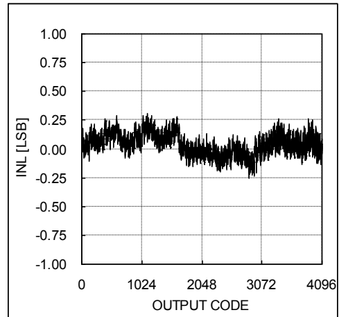
Figure 7. INL vs OUTPUT CODE ( V_A=3\text{V} , f_{SCLK}=10\text{MHz} , f_S=500\text{kSPS} )
