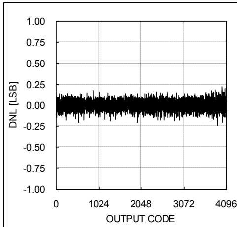
Figure 6. DNL vs OUTPUT CODE ( V_A=3\text{V} , f_{SCLK}=10\text{MHz} , f_S=500\text{kSPS} )
