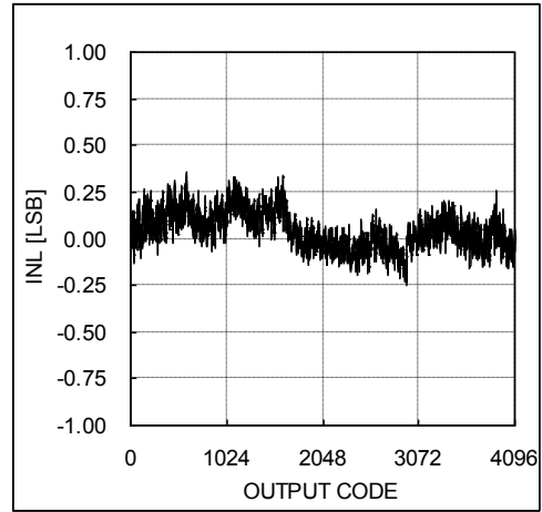
Figure 9. INL vs OUTPUT CODE ( V_A=3\text{V} , f_{SCLK}=20\text{MHz} , f_S=1\text{MSPS} )
