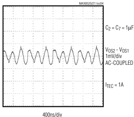
DIFFERENTIAL OUTPUT VOLTAGE RIPPLE
