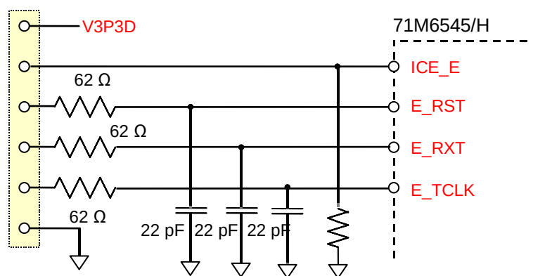
Figure 32: External Components for the Emulator Interface
