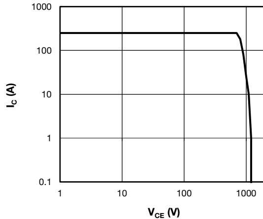
Fig. 16 - Trench IGBT Reverse BIAS SOA T_J = 150\text{ °C} , I_C = 250\text{ A} , R_g = 10\ \Omega , V_{GE} = +15\text{ V} / 0\text{ V} , V_{CC} = 700\text{ V} , V_p = 1200\text{ V}
