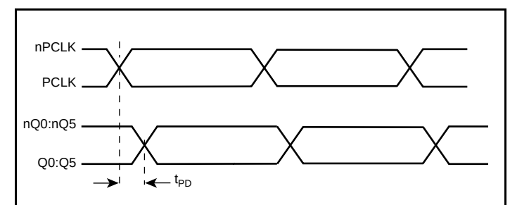
Propagation Delay
