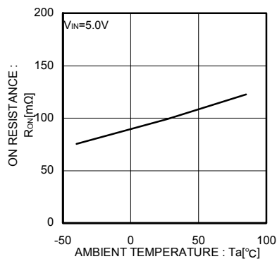
Fig.58 ON resistance
