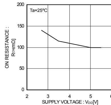
Fig.57 ON resistance
