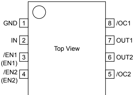
Fig.86 Pin Configuration
