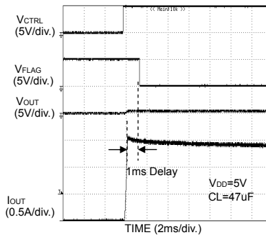
Fig.78 Over current response Enable to shortcircuit (BD6516F)
