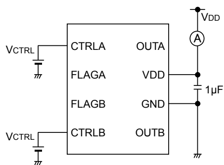
Operating current
