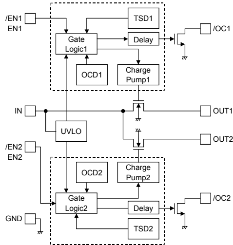
Fig.85 Block diagram
