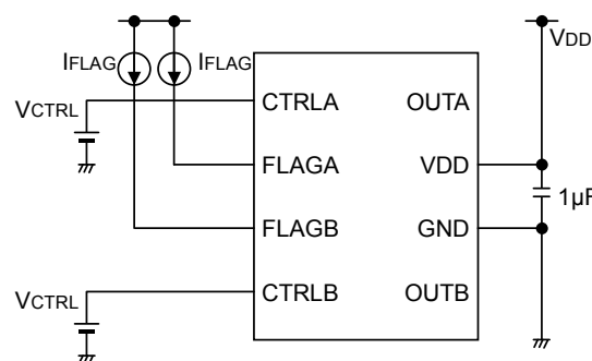
FLAG output resistance
