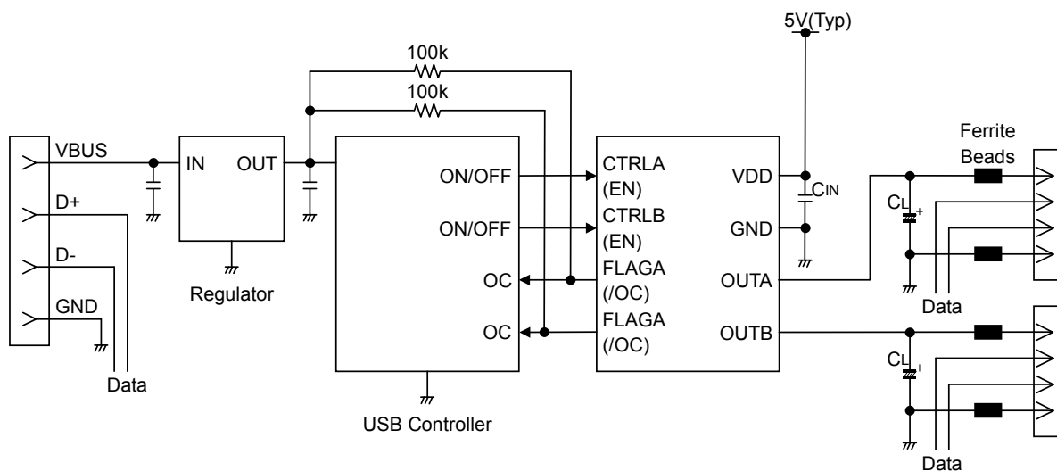
Fig.89 Typical application circuit
