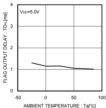
Fig.46 Flag output delay
