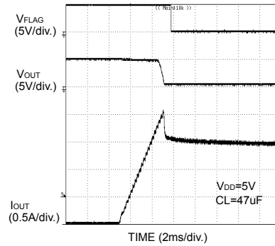
Fig.75 Over current response Ramped load (BD6516F)
