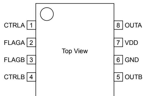
Fig.84 Pin Configuration
