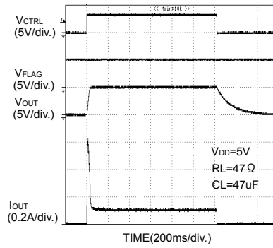
Fig.72 Output rise, fall characteristic (BD6516F)
