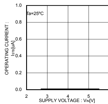
Fig.51 Operating current EN,/EN Disable
