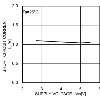
Fig.59 Output current at shortcircuit
