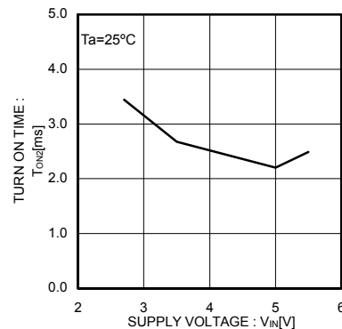
Fig.63 Output turn on time
