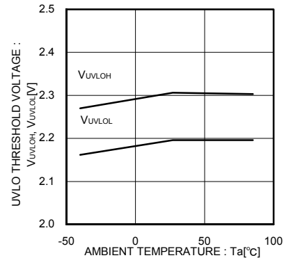
Fig.69 UVLO threshold voltage
