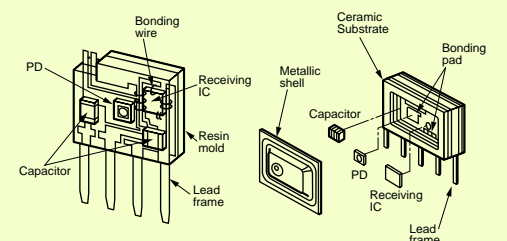
Molded resin package Ceramic package Structure of internal units
