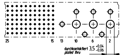
Board hole pattern (Component mounting side) for press fitting
