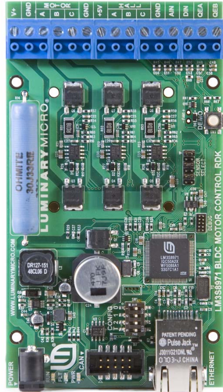
Figure 1. BLDC Motor Control Board
