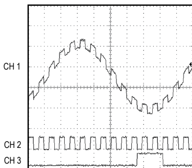
COMMON-MODE VOLTAGE FAULT (LOW SIDE)
