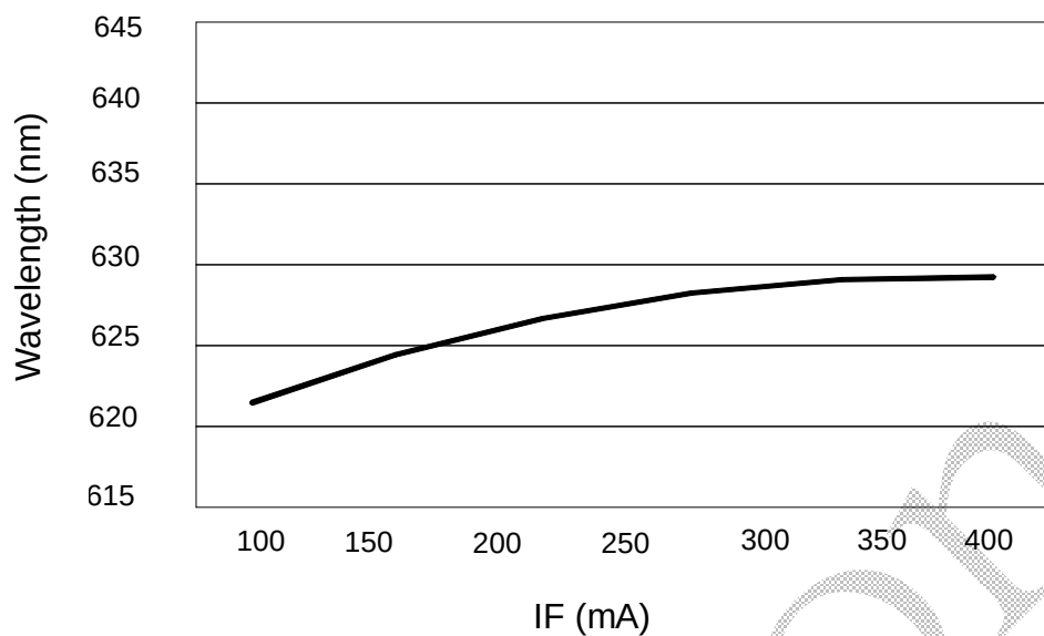
Forward Current VS Wavelength
