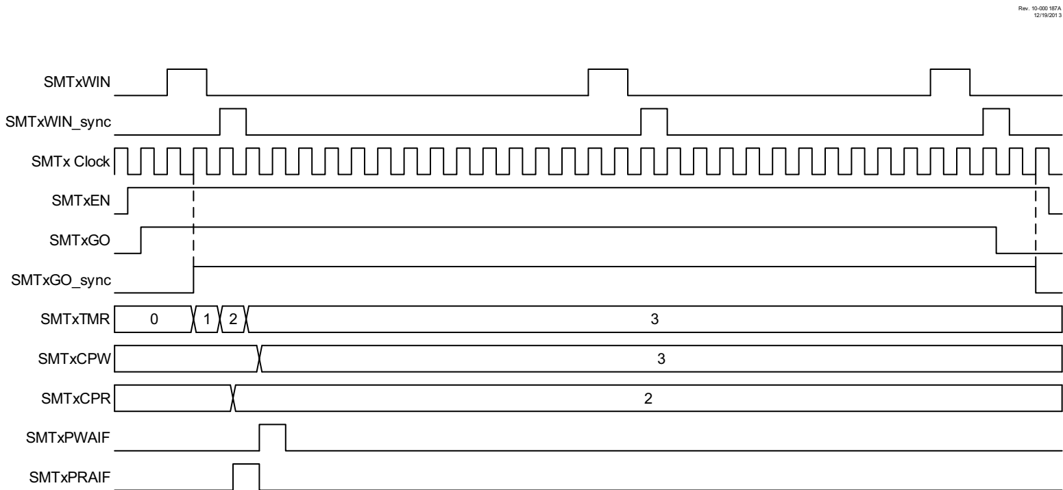
FIGURE 25-17: CAPTURE MODE SINGLE ACQUISITION TIMING DIAGRAM
