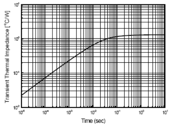
Fig.4 Thermal Response
