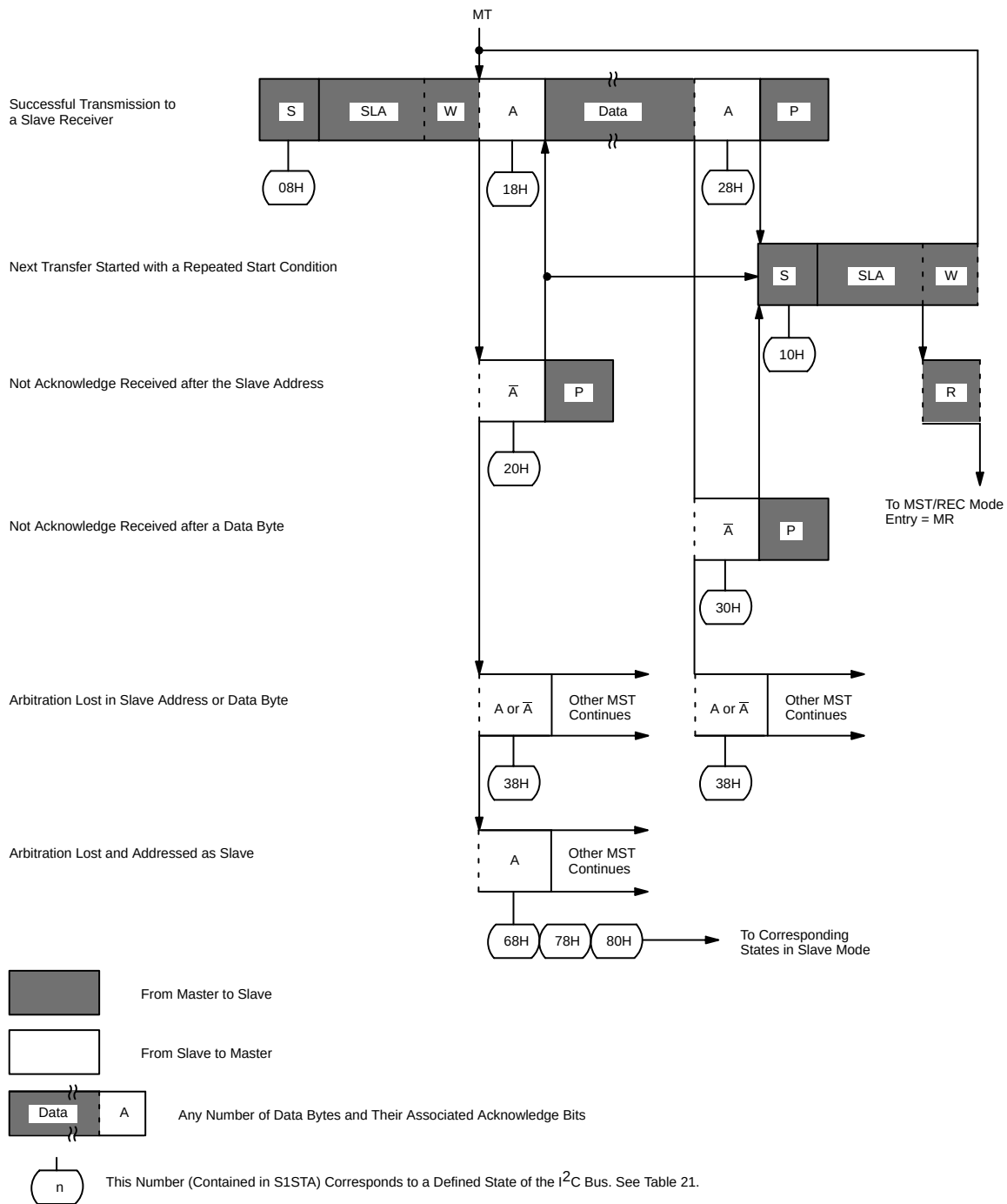
Figure 20. Format and States in the Master Transmitter Mode
