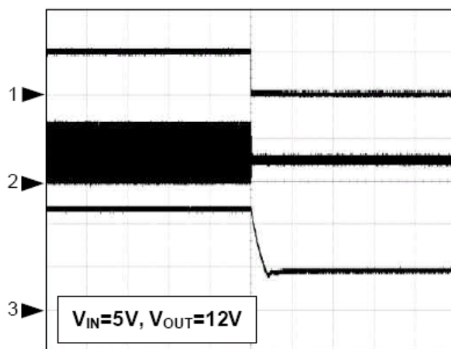
EN Goes Low - Shutdown, I_o=500mA
