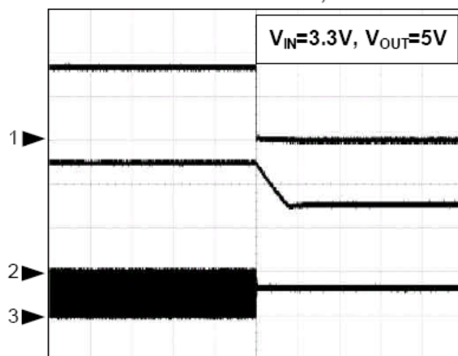
EN Goes Low - Shutdown, I_o=100mA
