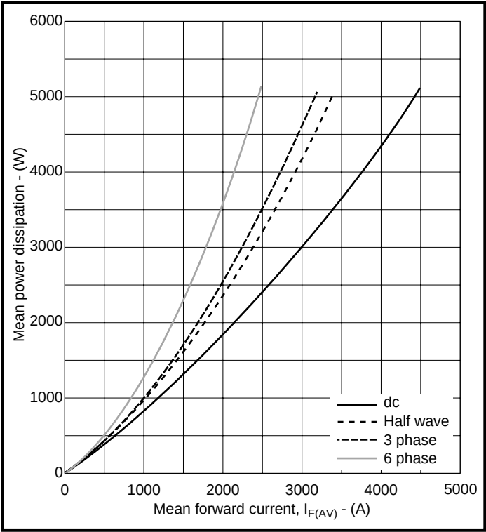
Fig.3 Dissipation curves
