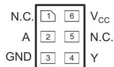
N.C. – No internal connection See mechanical drawings for dimensions. 图 5-2. DRY Package 6-Pin SON Transparent Top View
