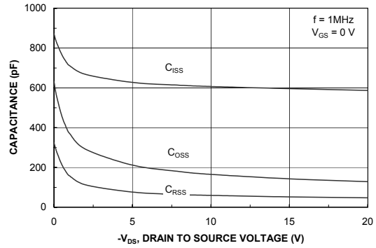
Figure 19. Capacitance Characteristics.
