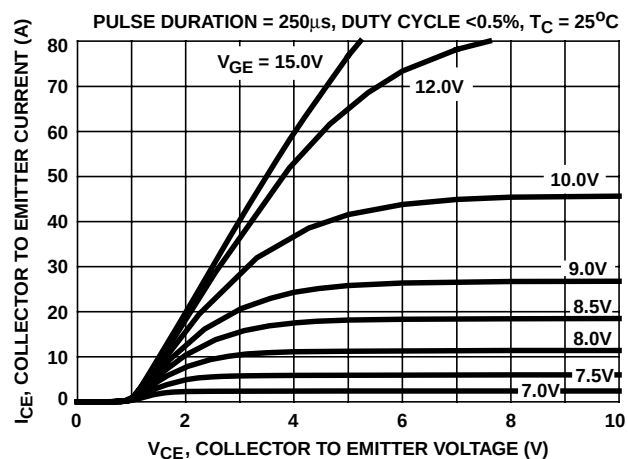
FIGURE 2. SATURATION CHARACTERISTICS
