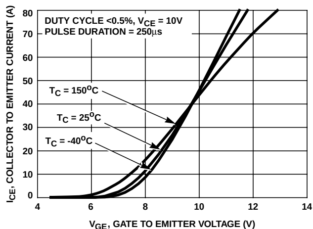
FIGURE 1. TRANSFER CHARACTERISTICS
