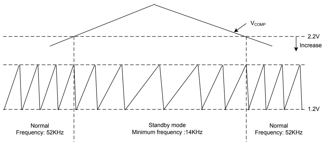
OSC triangle wave
