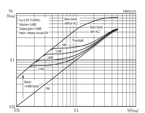
Figure 12. BASS ALC: Threshold curve
