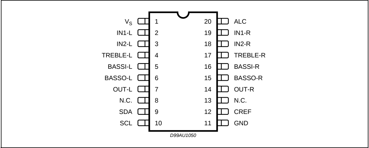
Figure 3. Pin Connection
