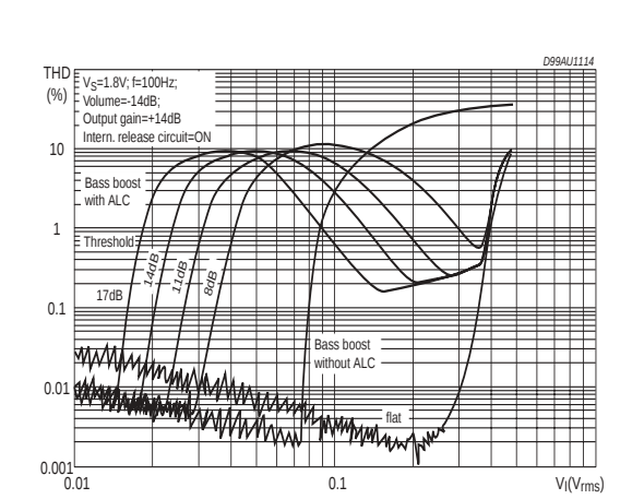
Figure 13. BASS ALC: THD
