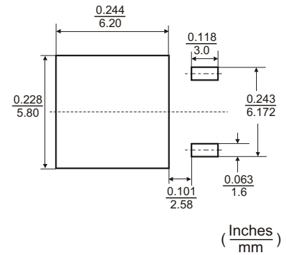
Pad Layout
