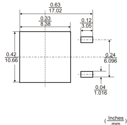
Pad Layout
