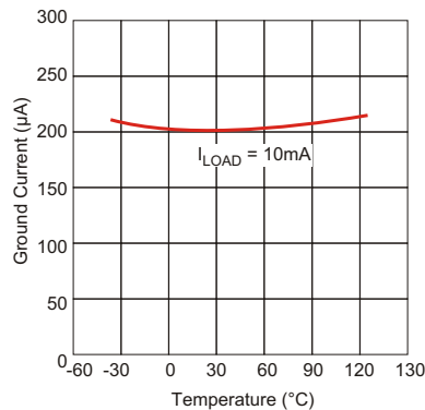
Figure 6. GM66102 Ground Current vs. Temperature
