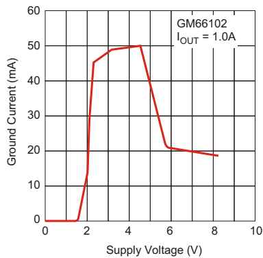
Figure 5. GM66102 Ground Current vs. Supply Voltage
