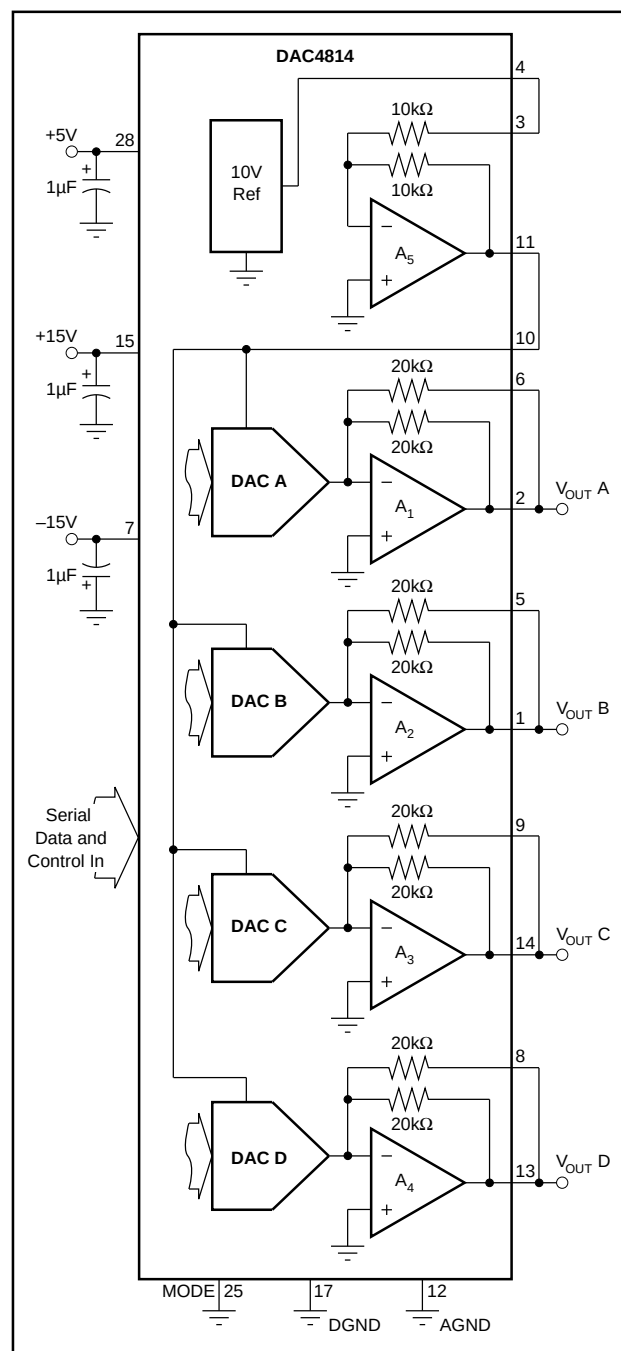
FIGURE 4. Analog Connections for 0 to +10\text{V} DAC Output.
