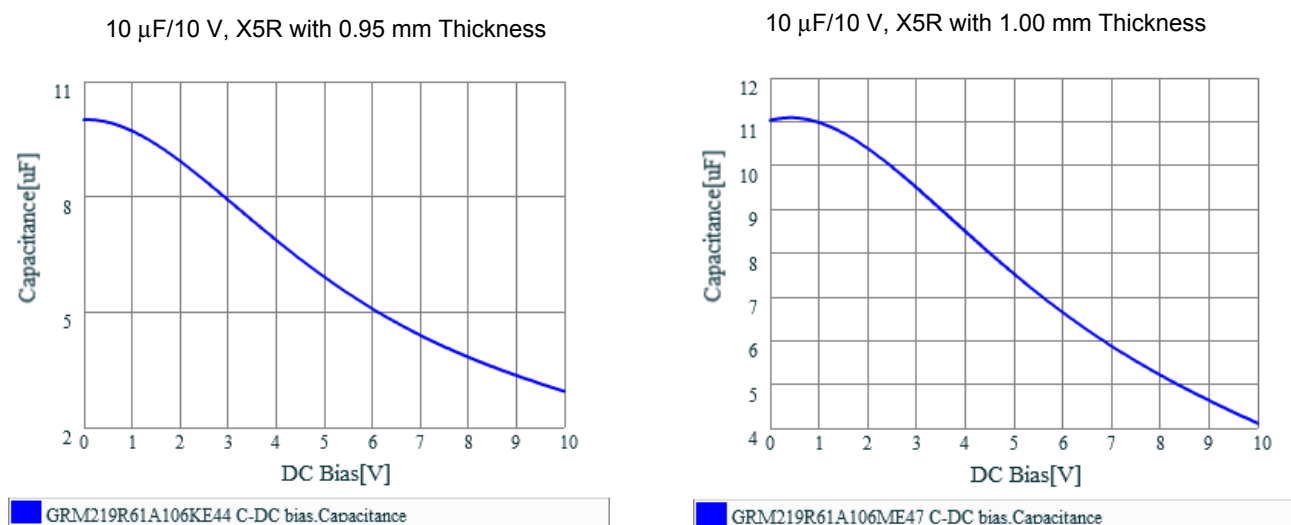
Figure 23. Capacitor DC bias
