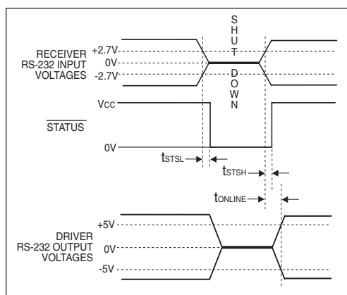
Figure 17. AUTO ON-LINE® Timing Waveforms
