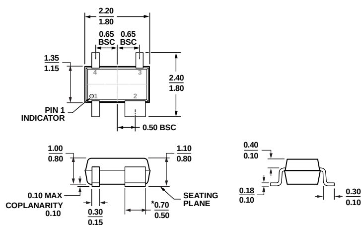
Figure 22. 4-Lead Thin Shrink Small Outline Transistor Package [SC70] (KS-4)
