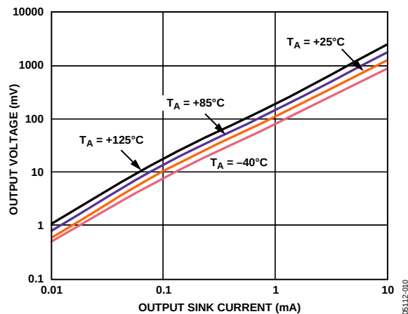
Figure 13. Output Voltage vs. Output Sink Current
