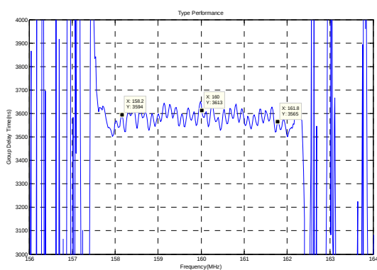
Group Delay Variation( f_0 \pm 1.8\text{MHz} )
