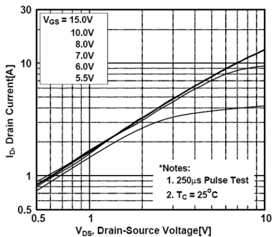
Fig. 1 On-State Characteristics
