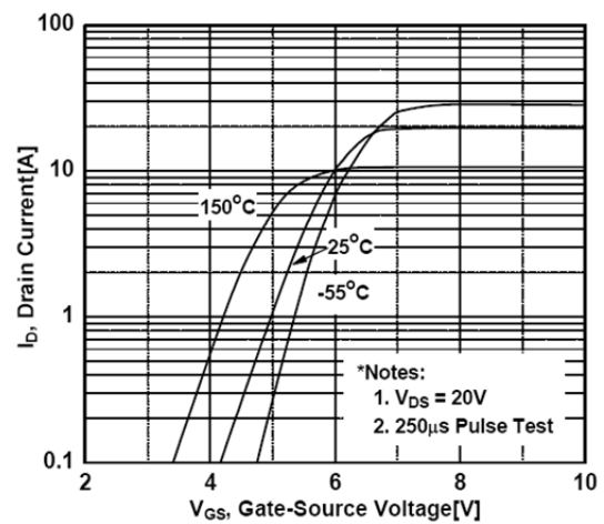
Fig. 2 Transfer Characteristics
