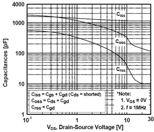
Fig. 5 Capacitance Characteristics
