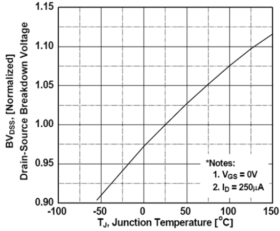
Fig. 3 Breakdown Voltage Variation vs Temperature
