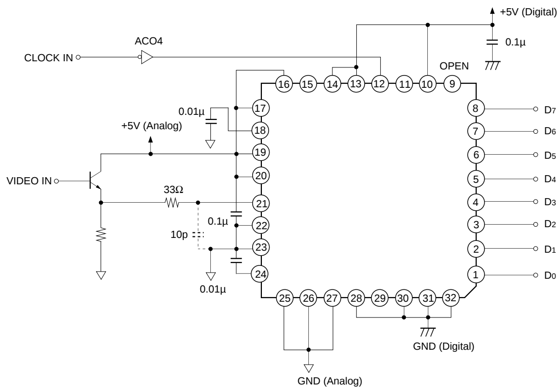
I-4. When clamp is used (self-bias not used)
