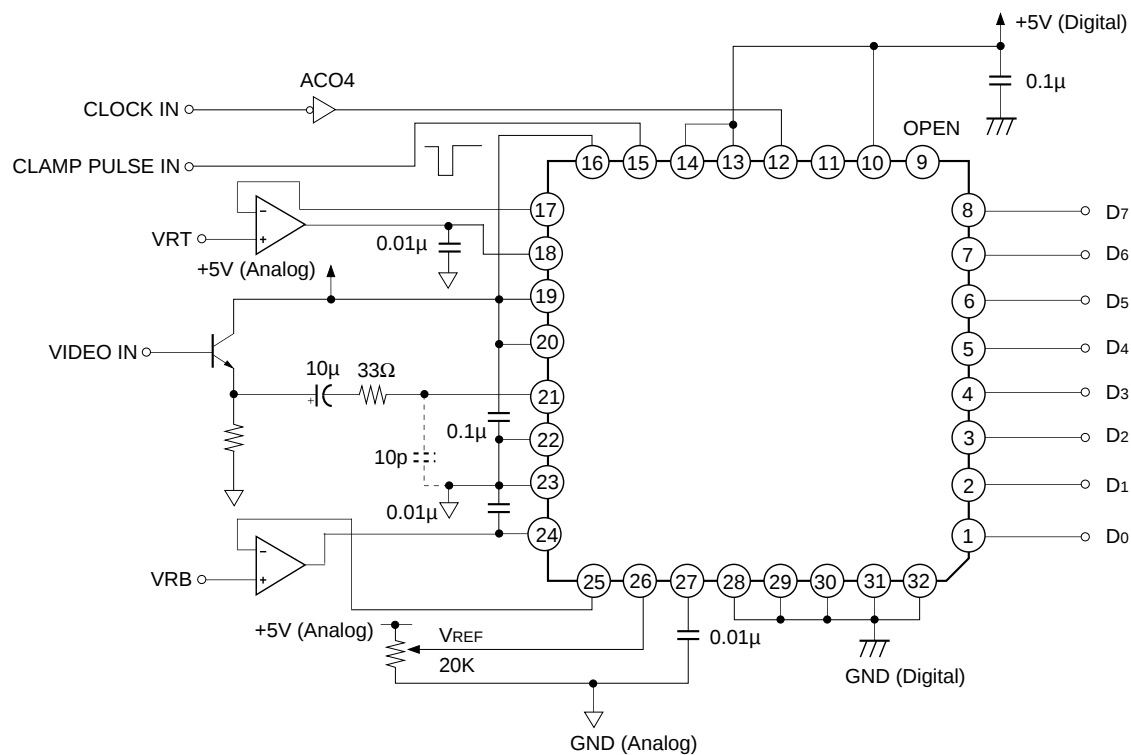
I-4. When clamp is used (self-bias not used)
