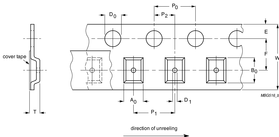
Fig. 6 Embossed Tape
