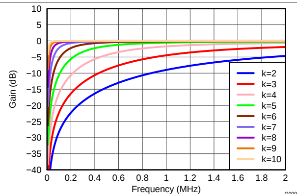
Figure 58. Digital HPF Response
