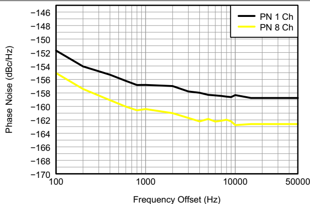
Figure 16. CW Phase Noise, F_{IN} = 2 MHz, 1 Channel vs 8 Channel
