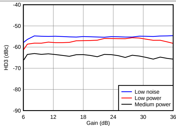
Figure 40. HD3 vs Gain, LNA = 15 dB and PGA = 24 dB and V_{OUT} = -1 dBFS
