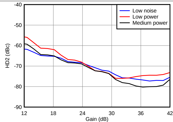
Figure 41. HD2 vs Gain, LNA = 18 dB and PGA = 24 dB and V_{OUT} = -1 dBFS
