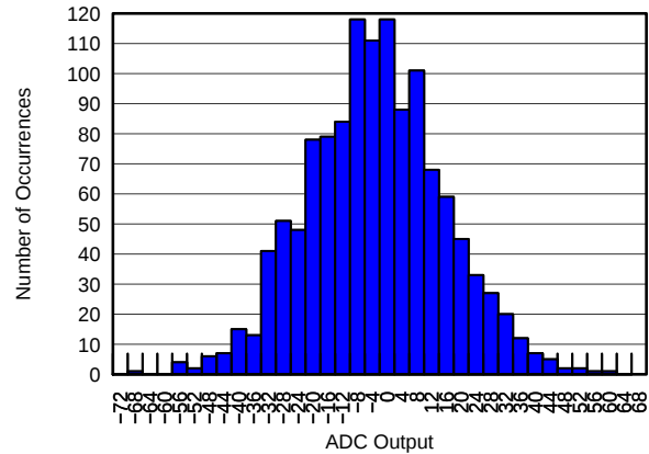
Figure 7. Output Offset Histogram, V_{\text{CNTL}} = 0 V (1247 Channels)
