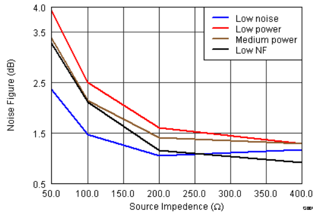
Figure 36. Noise Figure vs Power Modes Without Termination
