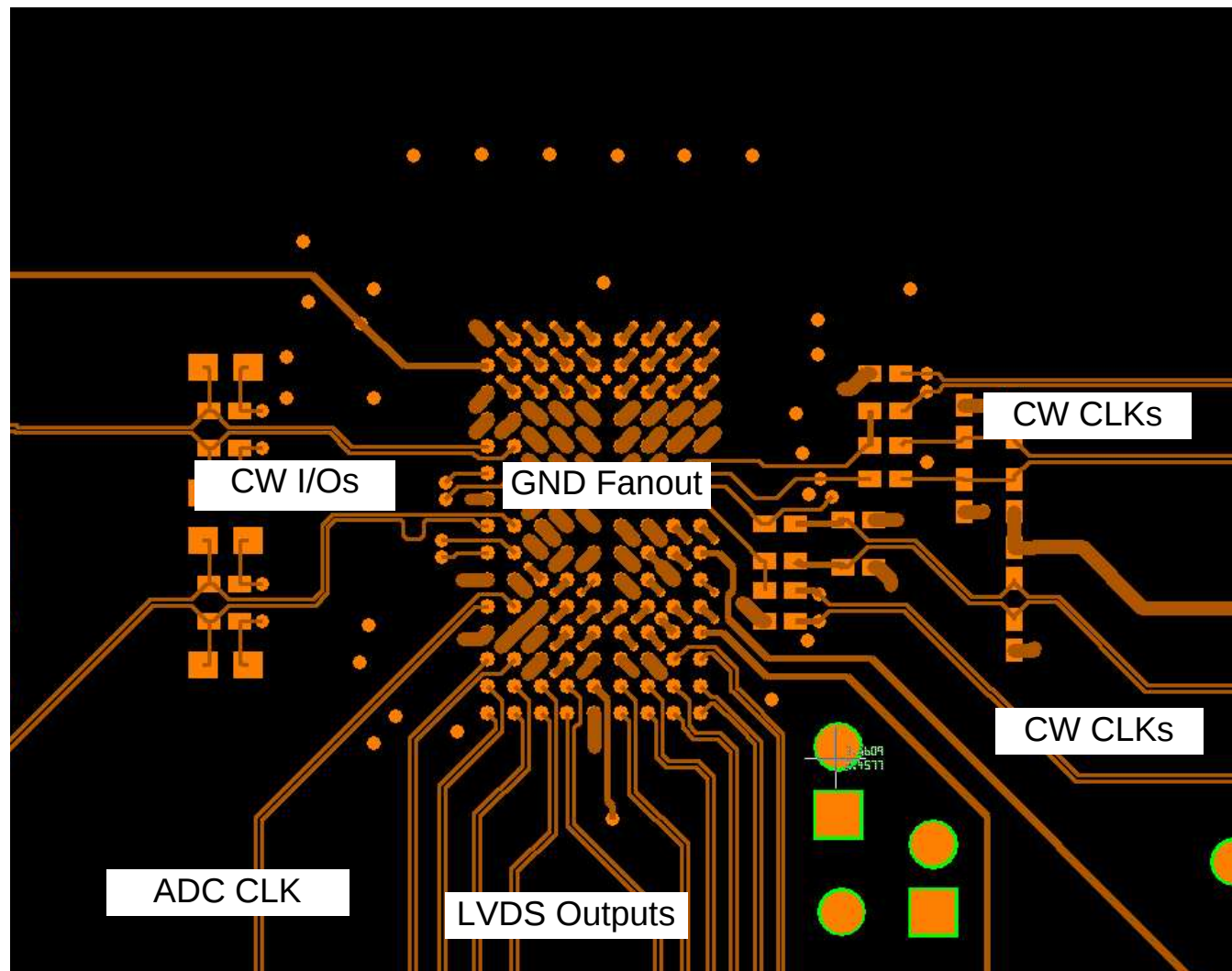
Figure 115. Layout Example
