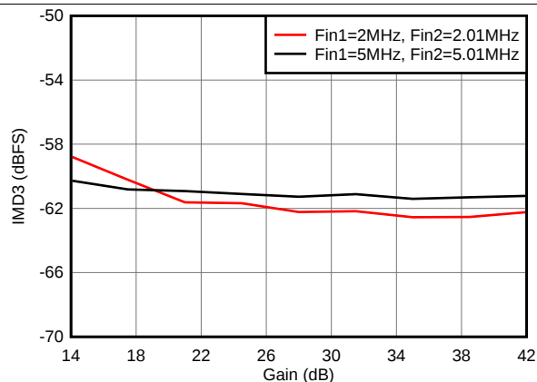
Figure 46. IMD3, Fout1 = -7 dBFS and Fout2 = -7 dBFS
