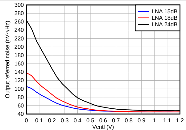
Figure 25. ORN, PGA = 24 dB and Medium-Power Mode
