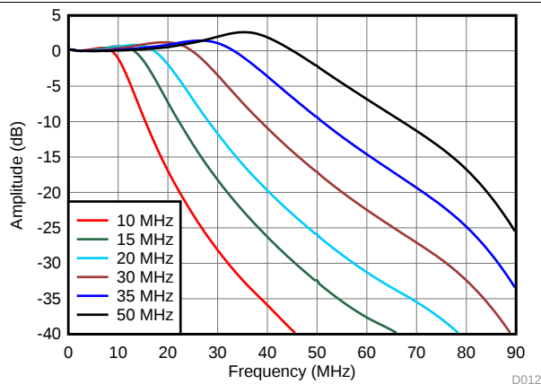
Figure 12. LPF Response
