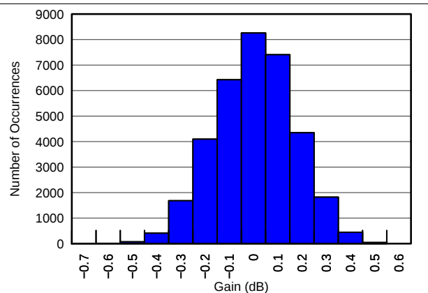
Figure 5. Gain Matching Histogram, V_{CNTL} = 0.6\text{ V} (34951 Channels)
