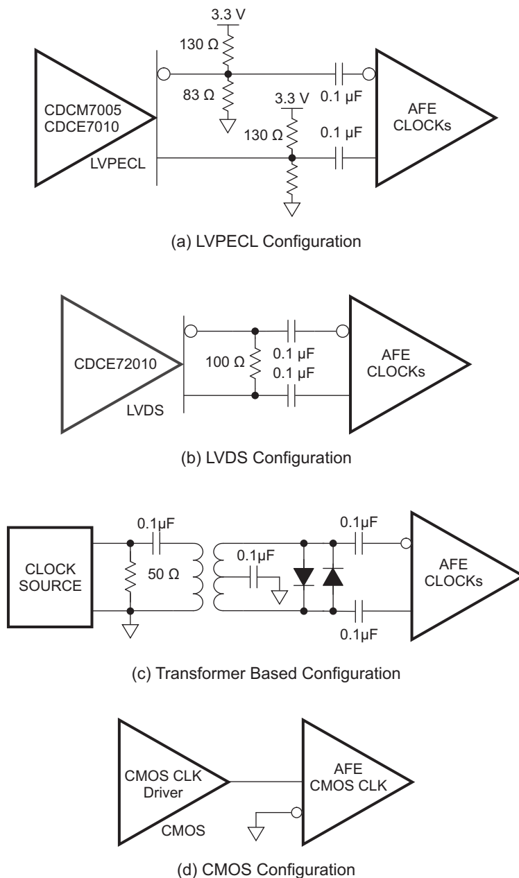
Figure 107. Clock Configurations
