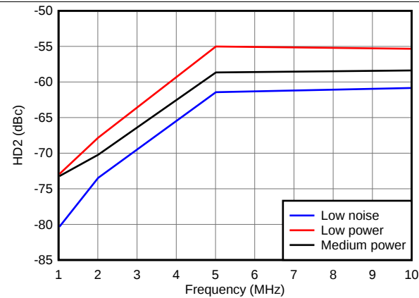
Figure 37. HD2 vs Frequency, V_{IN} = 500 mVpp and V_{OUT} = -1 dBFS
