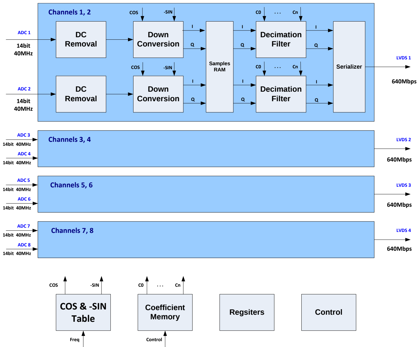
Figure 61. Digital Demodulator Block Diagram, M=4
