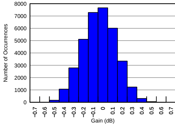
Figure 6. Gain Matching Histogram, V_{\text{CNTL}} = 0.9 V (34951 Channels)
