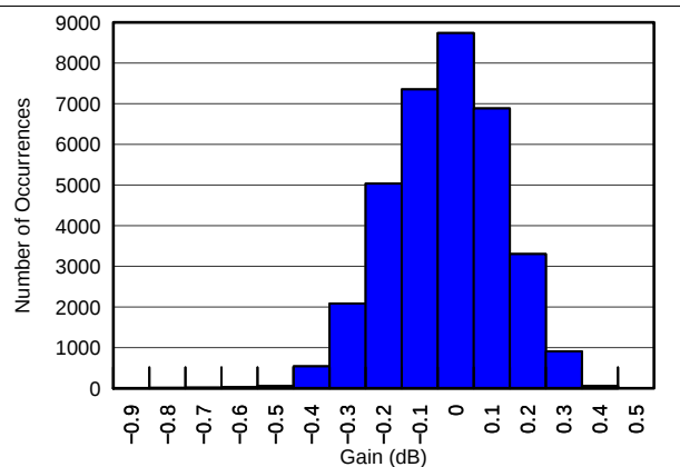
Figure 4. Gain Matching Histogram, V_{CNTL} = 0.3\text{ V} (34951 Channels)
