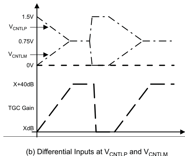
Figure 102. V_{CNTLP} and V_{CNTLM} Configurations
