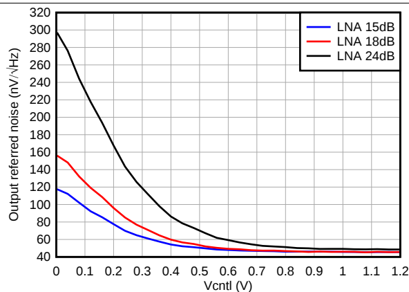
Figure 26. ORN, PGA = 24 dB and Low-Power Mode
