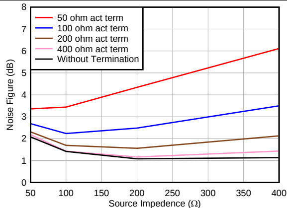
Figure 34. Noise Figure, LNA = 24 dB and Low Noise Mode
