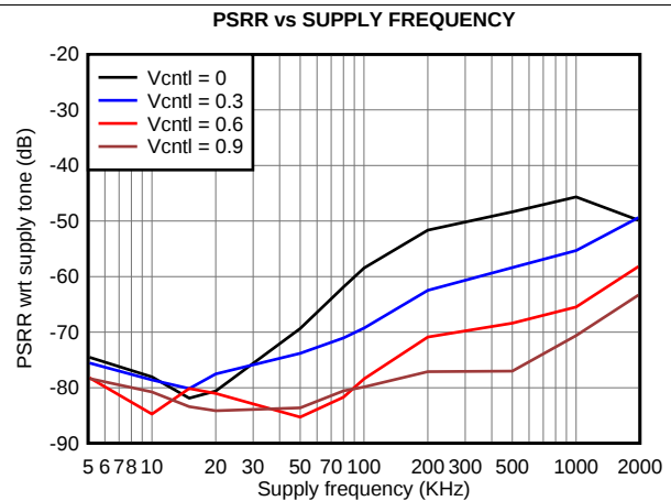
Figure 49. AVDD Power Supply Rejection Ratio, 100 mVpp Supply Noise With Different Frequencies
