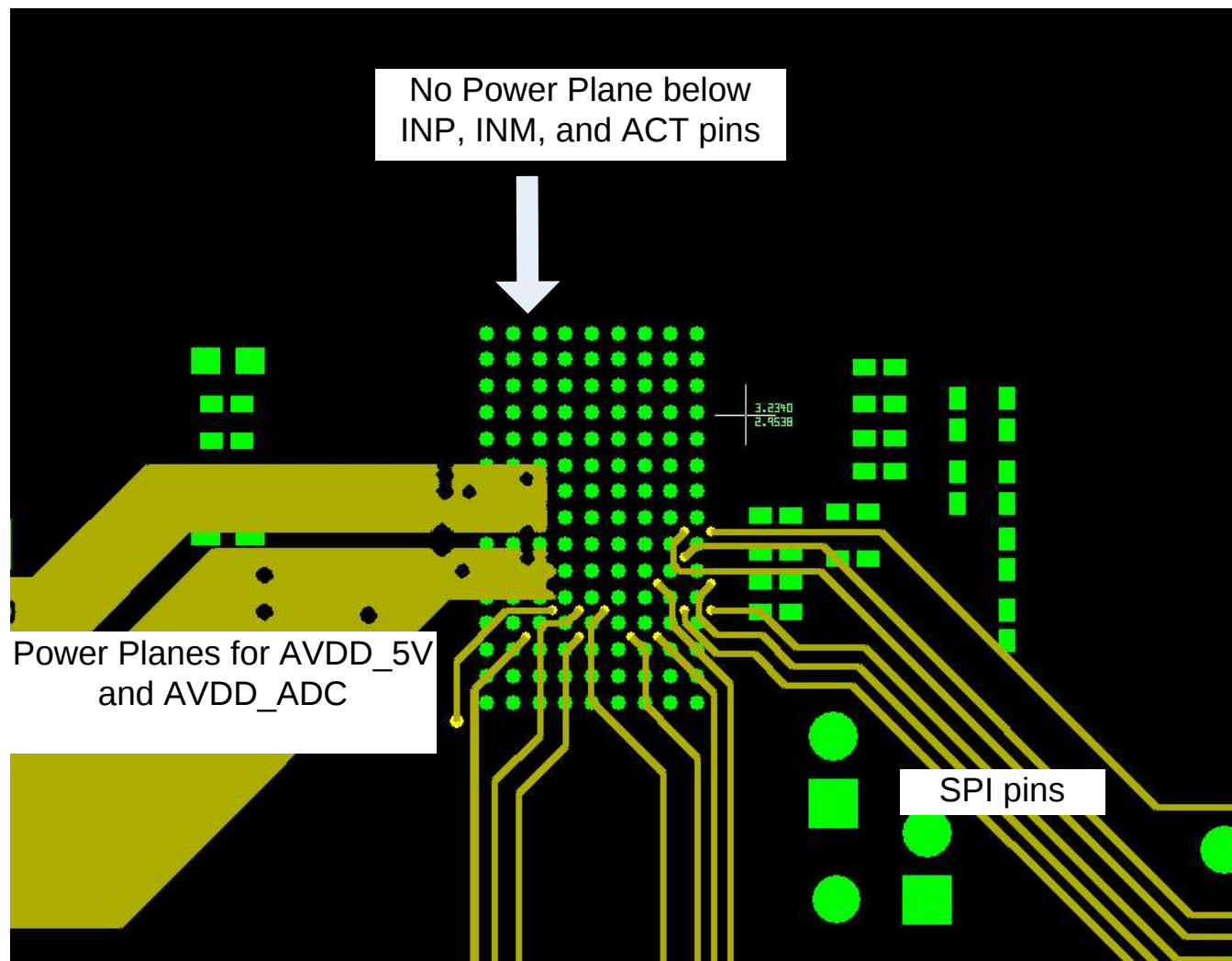
Figure 113. Layout Example
