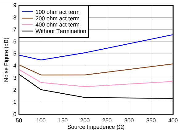
Figure 32. Noise Figure, LNA = 15 dB and Low Noise Mode
