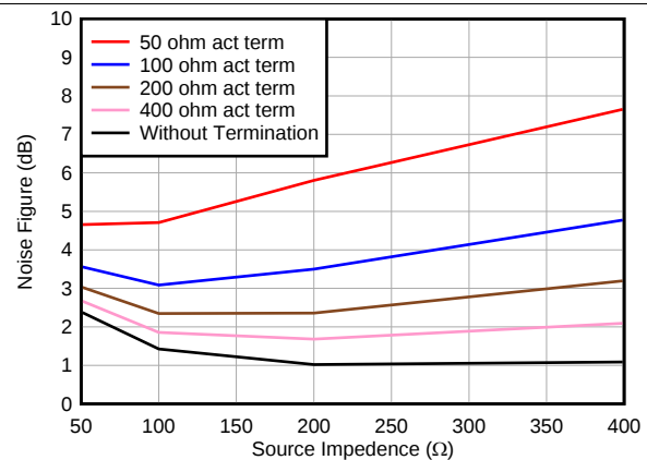
Figure 33. Noise Figure, LNA = 18 dB and Low Noise Mode
