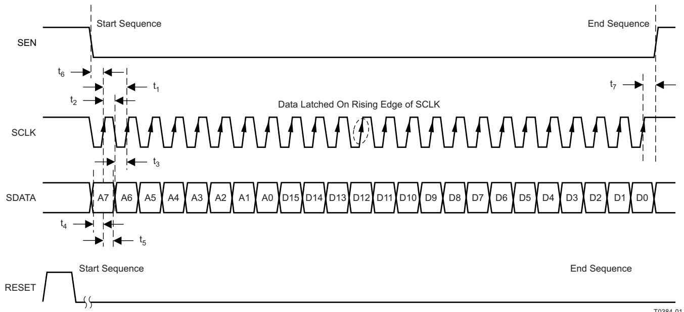
Figure 84. SPI Timing
