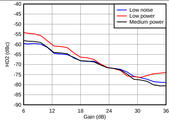
Figure 39. HD2 vs Gain, LNA = 15 dB and PGA = 24 dB and V_{OUT} = -1 dBFS
