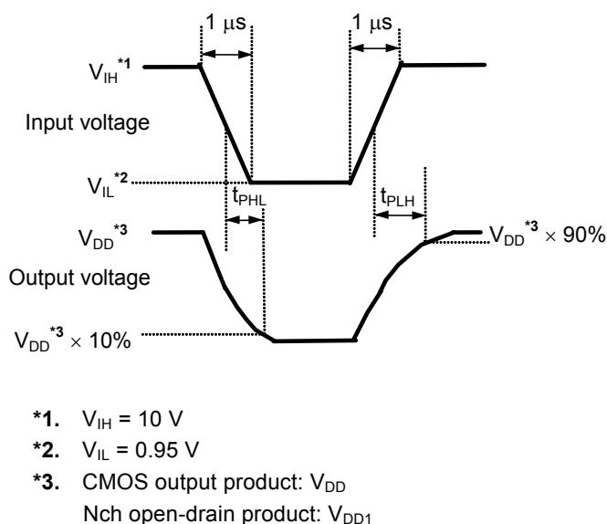
Figure 34 Test Condition of Response Time
