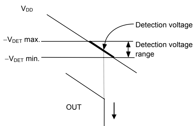
Figure 28 Detection Voltage
