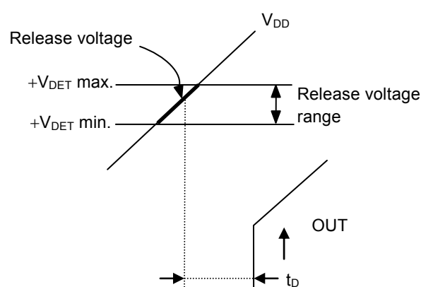
Figure 29 Release Voltage
