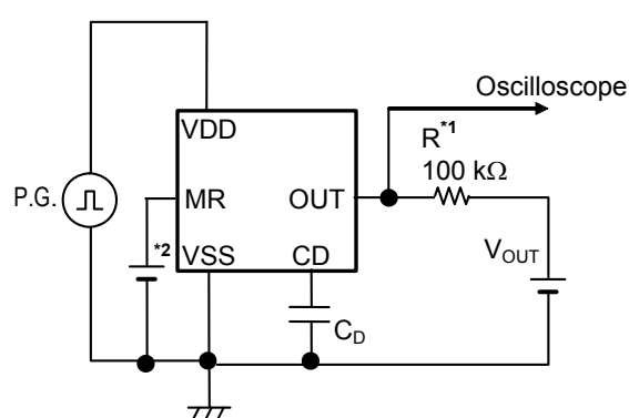
Figure 9 Test Circuit 2
