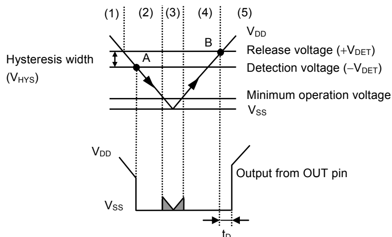
Figure 16 Operation 1
