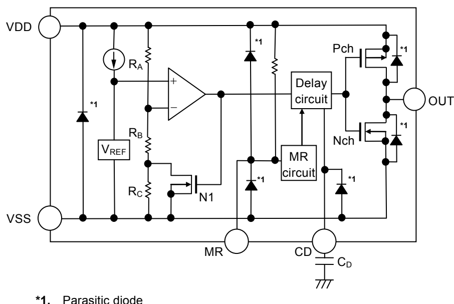
Figure 16 Operation 1
