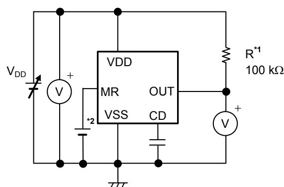
Figure 28 Detection Voltage
