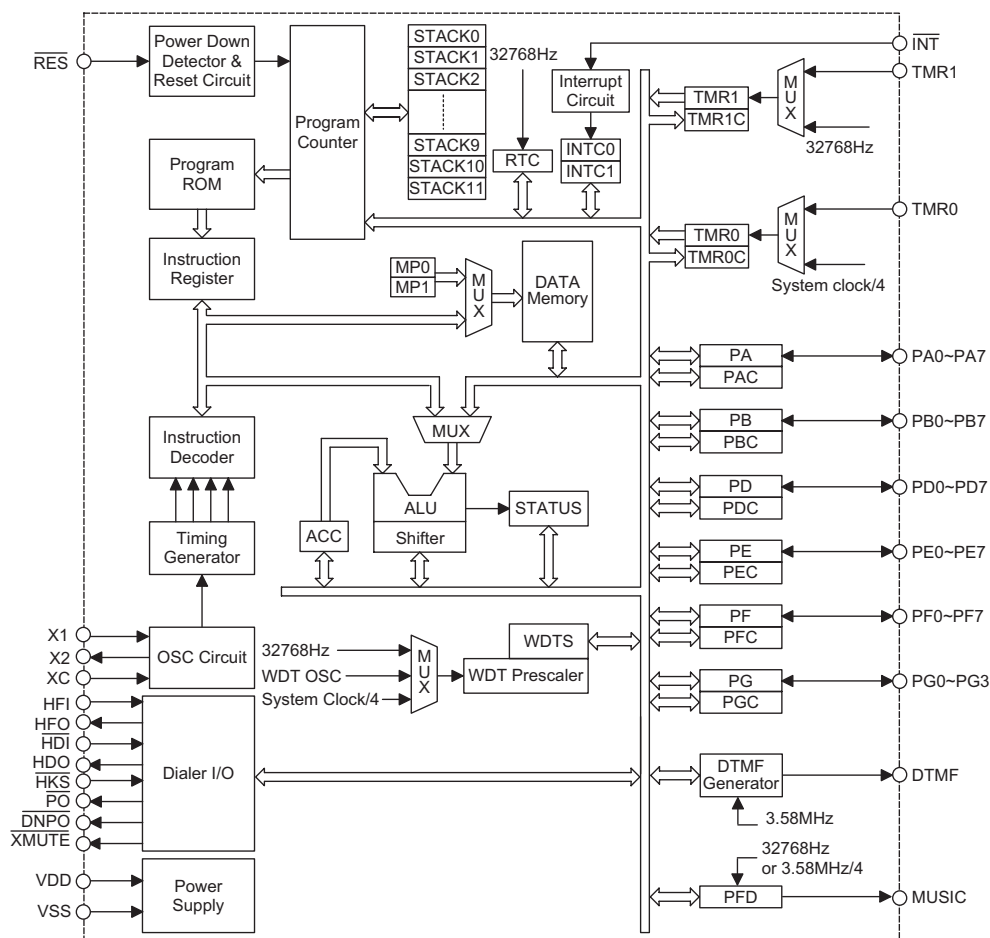
Block Diagram (HT95A400/40P)
