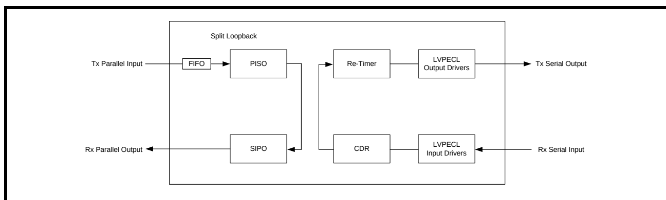
FIGURE 21. SPLIT LOOPBACK
