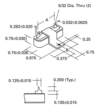
Printed Circuit Terminal
