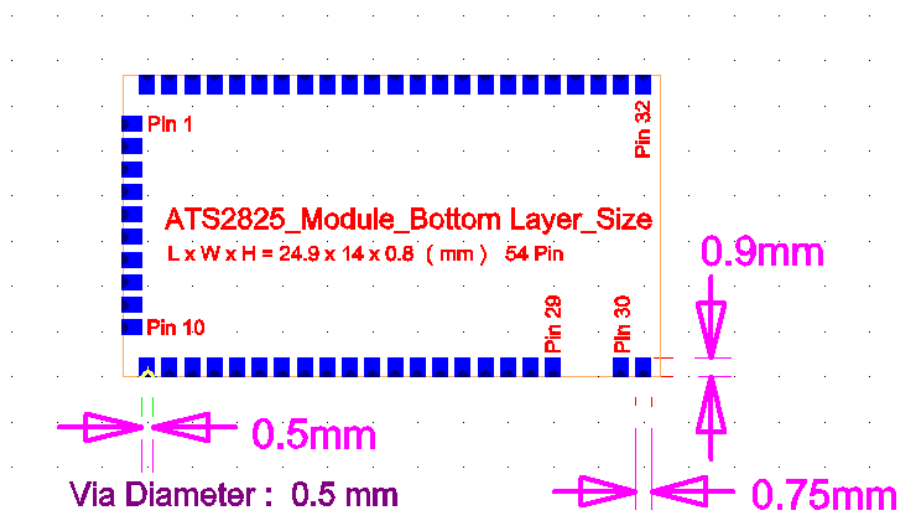
Module Dimension (Bottom VIEW)
