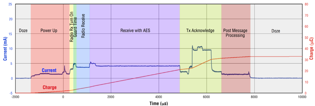
Atomic Operation - Maximum Length Receive with Acknowledge Pout=8dBm, 7.25ms Time Slot (32.6 \mu C Total Charge at 3.6V)
