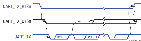
Figure 16. UART Mode 2 Transmit Flow Control
