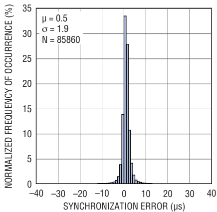
TIME n Synchronization Error 1 Packet/s Publishing Rate, 1 Hop, 2°C/Min
