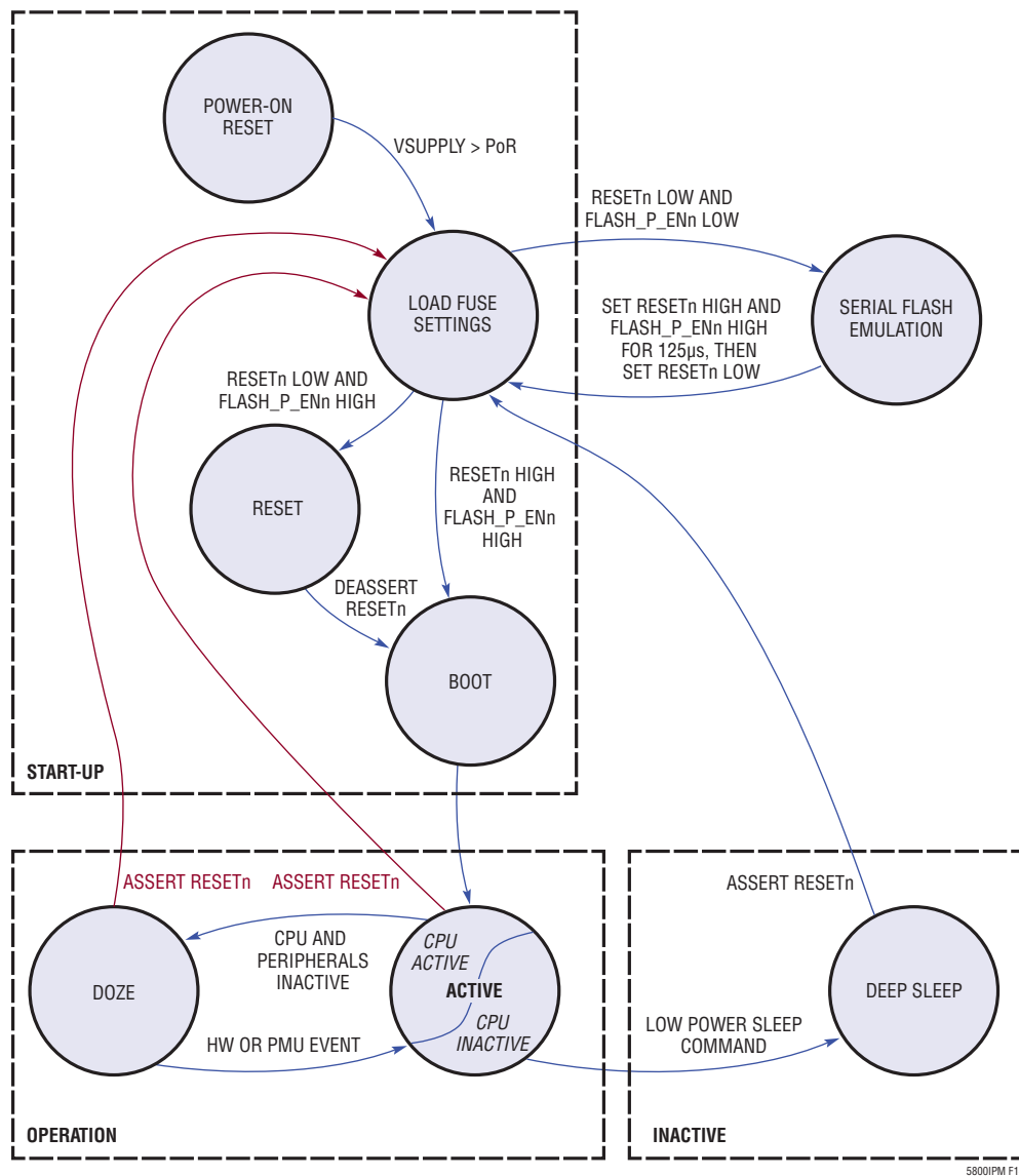
Figure 18. Eterna State Diagram
