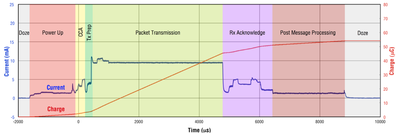
Atomic Operation - Maximum Length Transmit at Pout=8dBm with Acknowledge, 7.25ms Time Slot (54.5 \mu C Total Charge at 3.6V)
