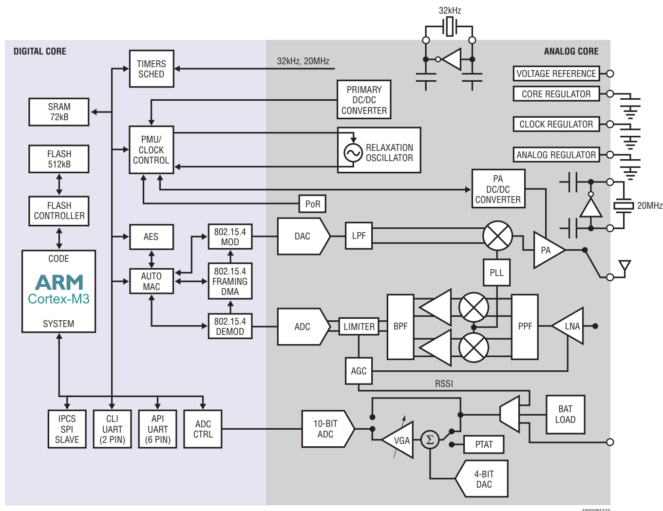
Figure 14. Eterna Block Diagram
